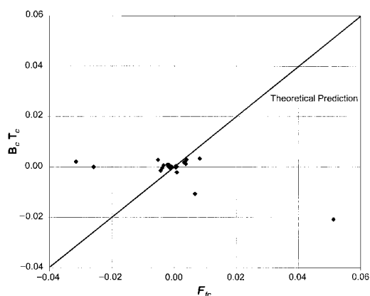
FIGURE 3. MEASURED FACTOR TRADE USING OWN TECHNOLOGY MATRIX VERSUS ACTUAL FACTOR TRADE
